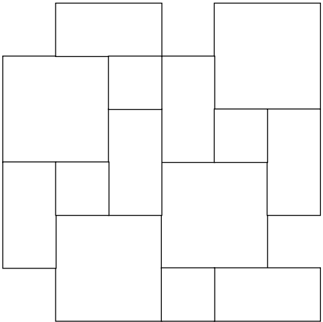
ROMAN PATTERN (4) 12x12,(6) 6x12, (4) 6x6, 8 SF
